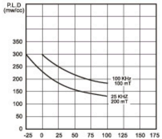
Power Loss v.s Temperature
