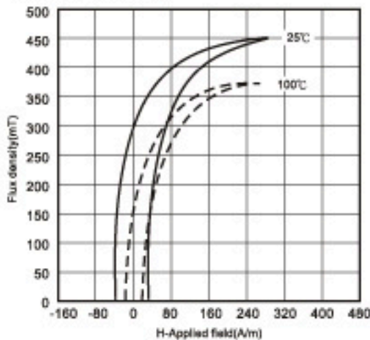
Magnetization Curve
