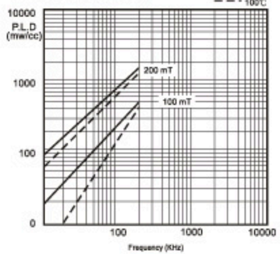
Power Loss v.s Frequency
