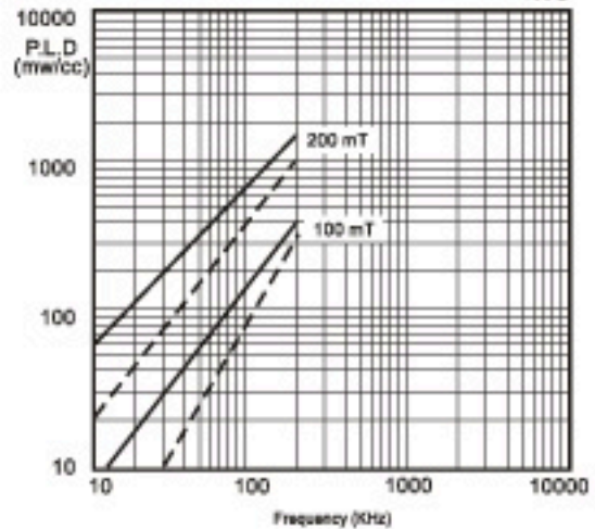
Power Loss v.s Frequency
