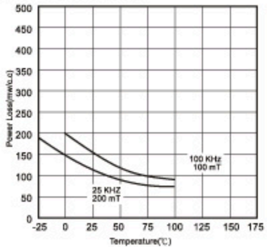
Power Loss v.s Temperature
