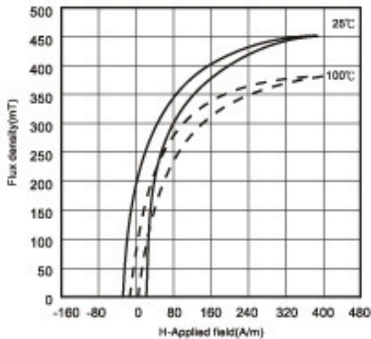
Magnetization Curve
