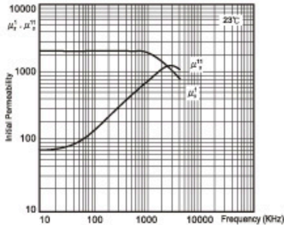
Complex Permeability vs. Frequency
