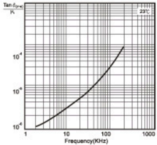
Relative Loss Factor vs. Frequency
