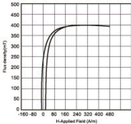
Magnetization Curve
